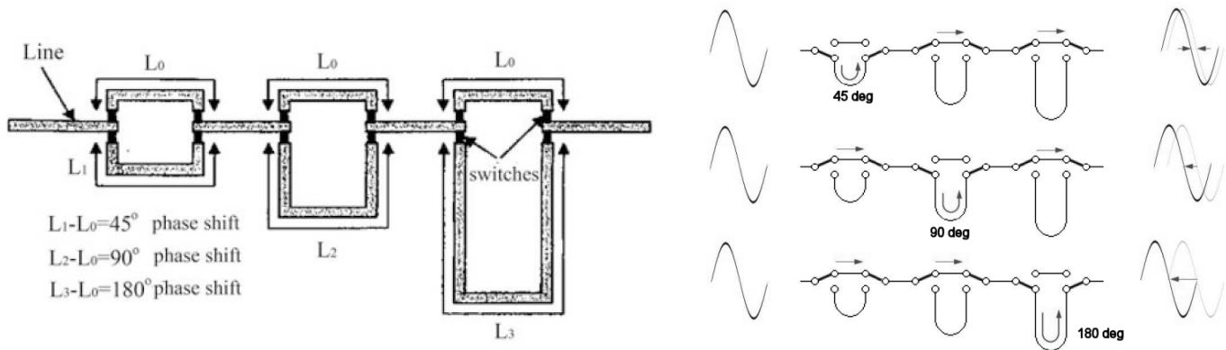
Three-Bit switched-line phase shifter and Signal Path
