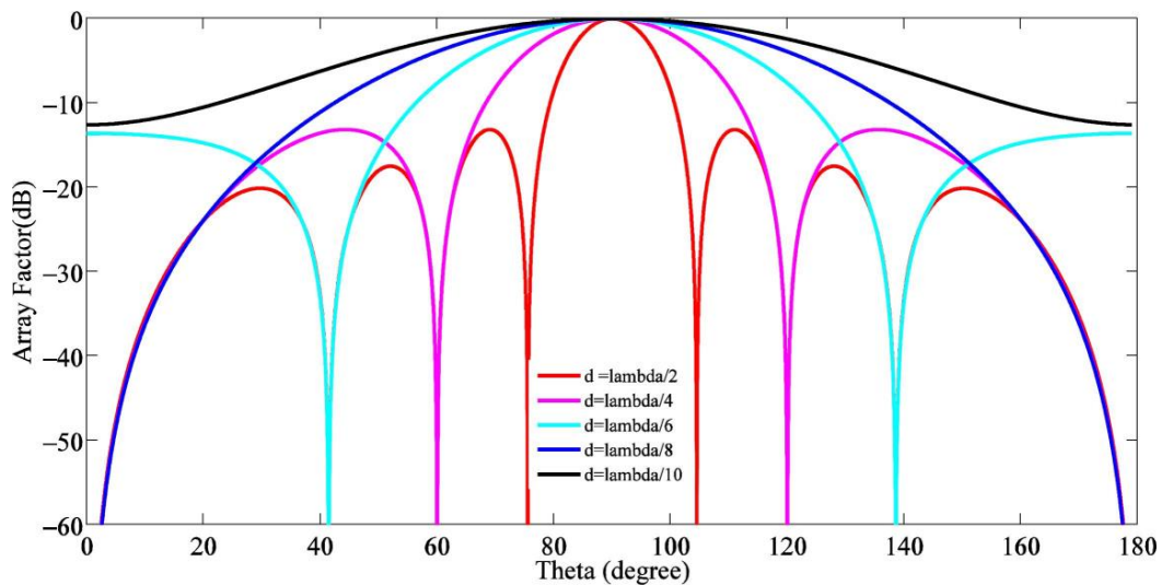
Array Factor (AF) varied with distance, d decreasing from \lambda/2 to \lambda/10
