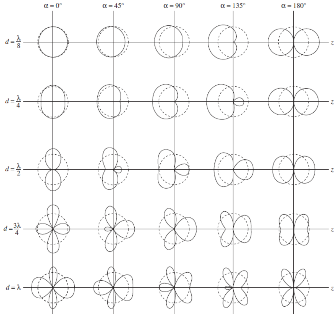
Patterns of Phased Array Antennas with two isotropic elements
