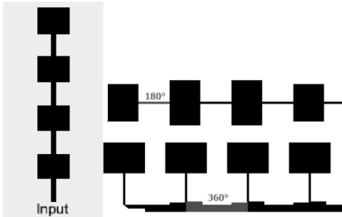
Series Feeding Linear Arrays
