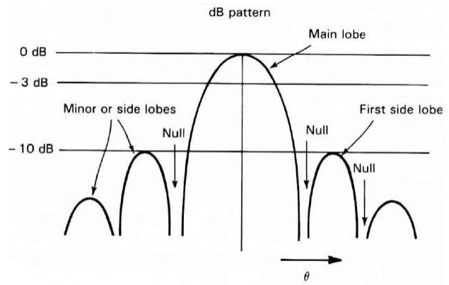
Antenna pattern in polar 2D coordinates Antenna pattern in rectangular coordinates in dB
