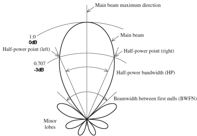
Antenna pattern in polar 2D coordinates Antenna pattern in rectangular coordinates in dB
