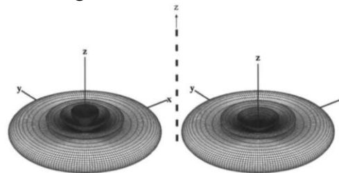
(isotropic elements) (Hertzian dipole elements)
