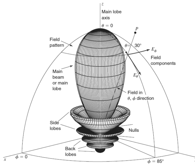
Antenna fields pattern in 3D coordinates
