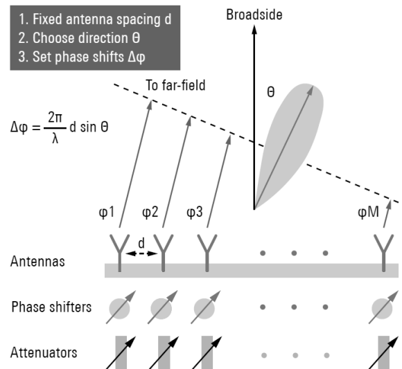
Scanned beam array block diagrams
