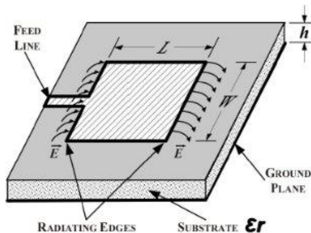
Patch Antenna with direct feed connection
