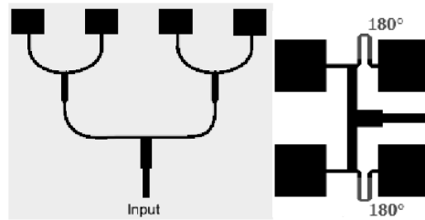
Corporate (Parallel) Feeding Linear Arrays
