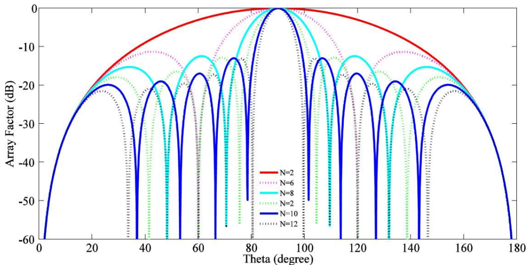
Array Factor (AF) varied with number of elements (N from 2 to 12)
