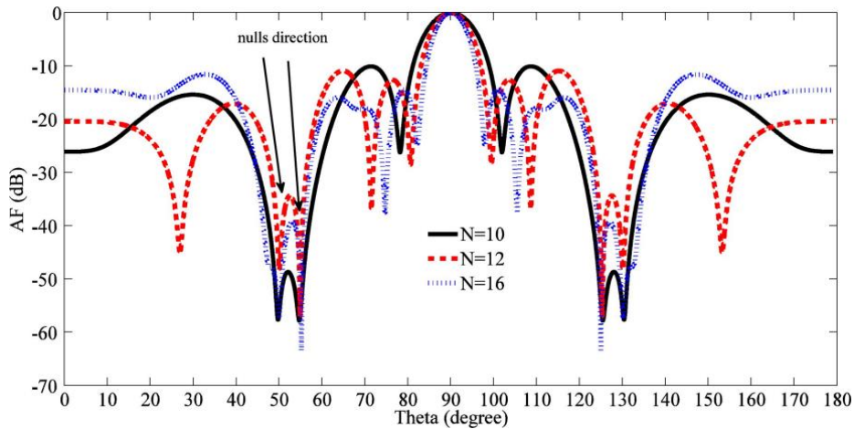
Array Factor (AF) when nulls are imposed at \theta=50^\circ, 55^\circ, 125^\circ, \text{ and } 130^\circ
