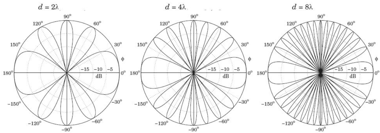
Grating lobes of two-element antenna array
